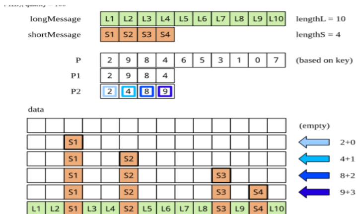
Fig. 8 Example of algorithm 1
